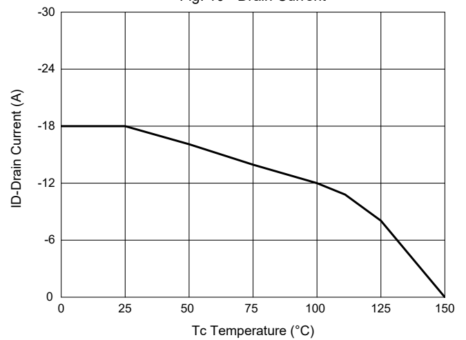
Fig. 10 - Drain Current
