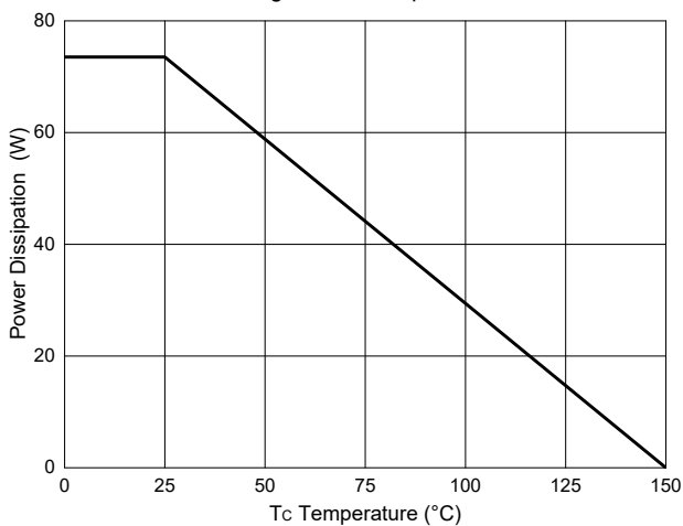
Fig.11-PD Dissipation
