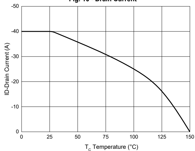
Fig. 10 - Drain Current
