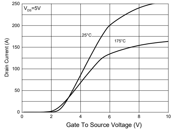
Fig. 2 - Transfer Characteristics
