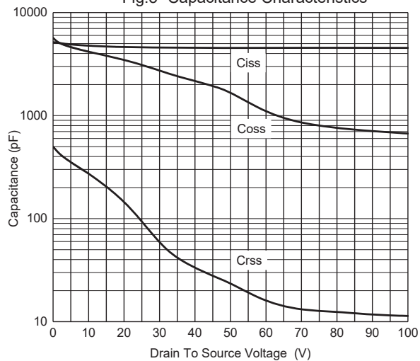
Fig.5- Capacitance Characteristics
