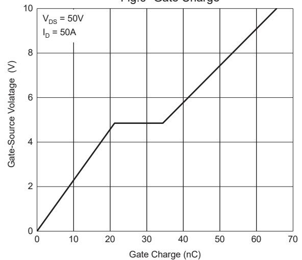
Fig.6- Gate Charge
