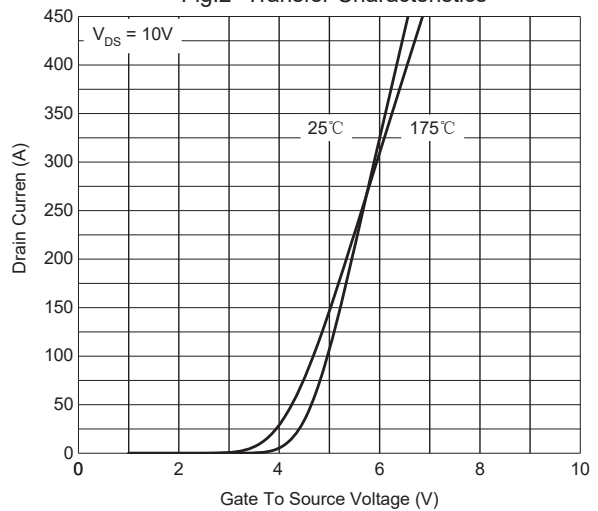
Fig.2- Transfer Characteristics
