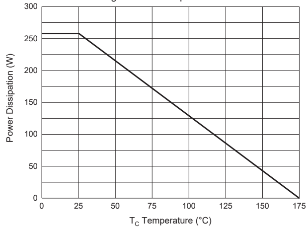
Fig. 11 - PD Dissipation
