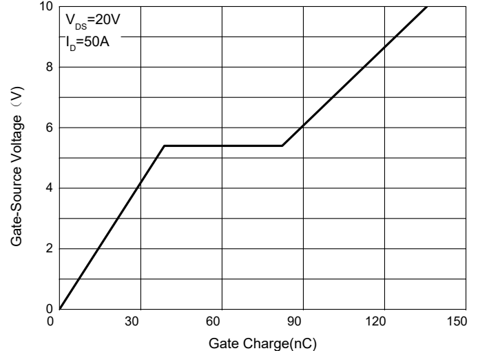
Fig. 6 - Gate Charge
