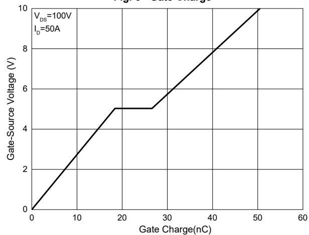
Fig. 6 - Gate Charge
