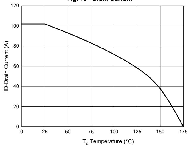
Fig. 10 - Drain Current
