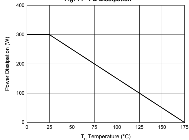
Fig. 11 - PD Dissipation
