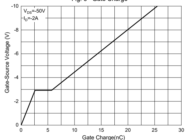
Fig. 6 - Gate Charge
