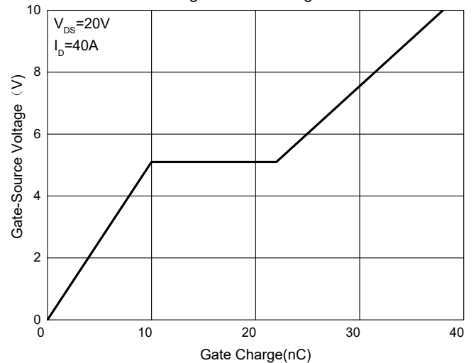
Fig. 6 - Gate Charge
