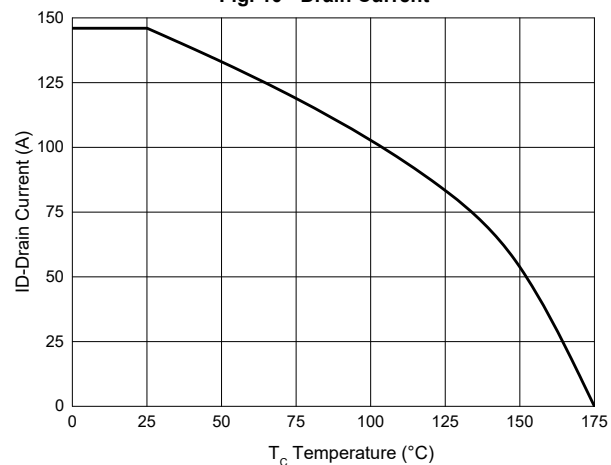
Fig. 10 - Drain Current
