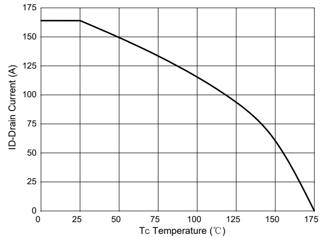
Fig. 10 - Drain Current
