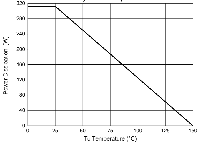
Fig.11-PD Dissipation
