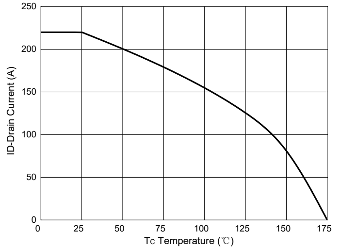
Fig. 10 - Drain Current
