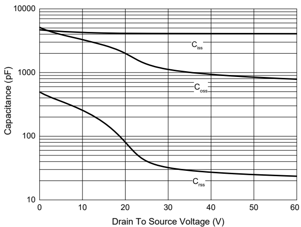
Fig. 5 - Capacitance Characteristics
