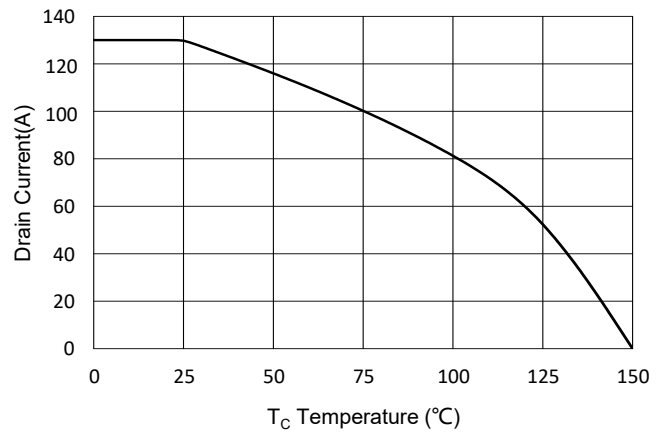
Fig.10 - Drain Current
