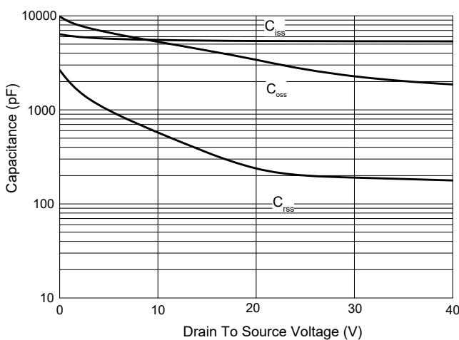
Fig.5 - Capacitance Characteristics
