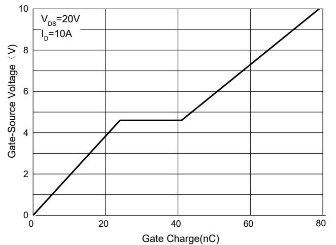
Fig.6 - Gate Charge
