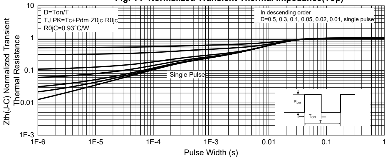
Fig. 14 -Normalized Transient Thermal Impedance(Top)
