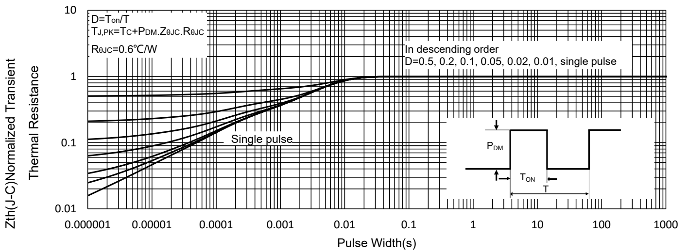
Fig.13 Normalized Transient Thermal Impedance
