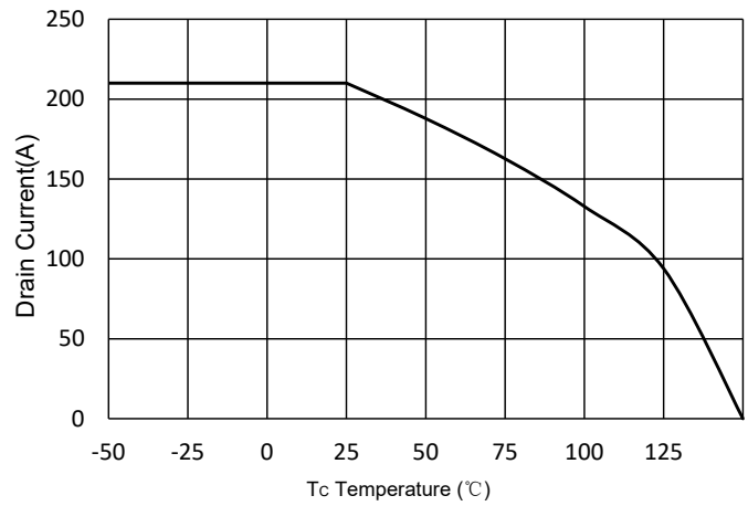
Fig.10 Drain Current
