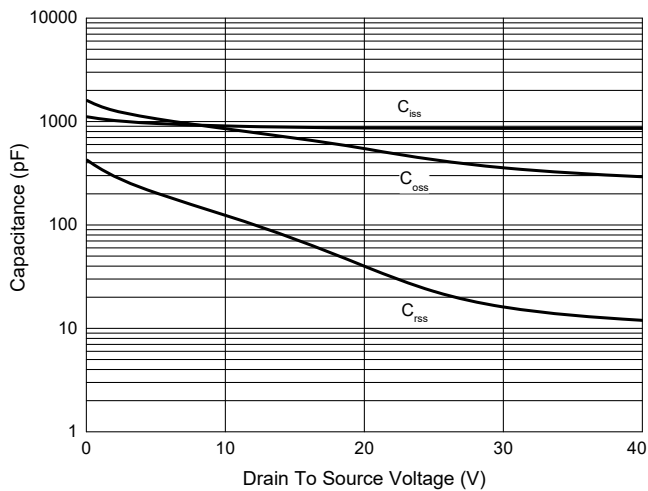
Fig. 5 - Capacitance Characteristics
