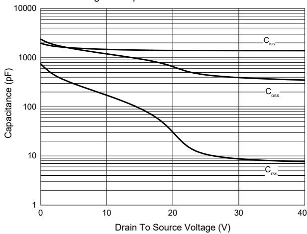
Fig. 5 - Capacitance Characteristics
