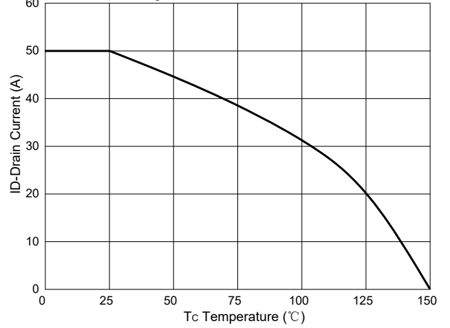
Fig. 10 - Drain Current
