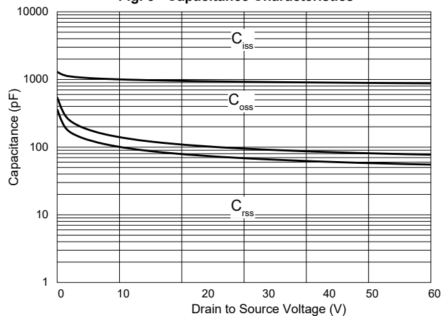
Fig. 5 - Capacitance Characteristics
