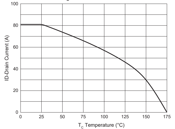
Fig. 10 - Drain Current
