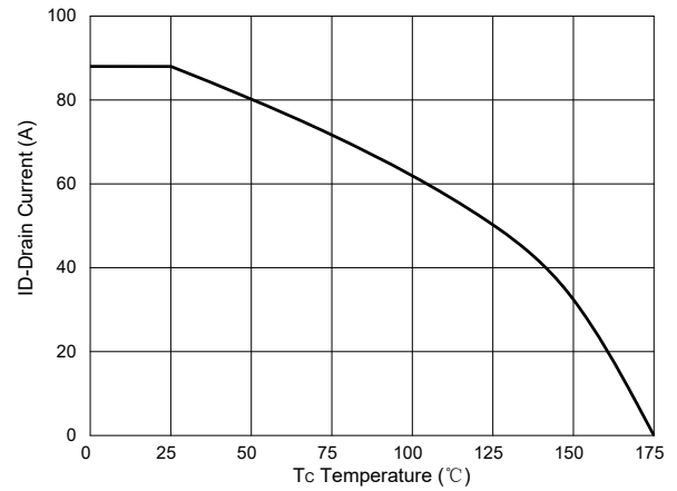
Fig.10 - Drain Current
