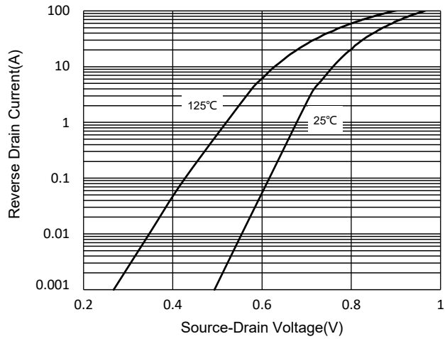
Fig.9-IS-VSD
