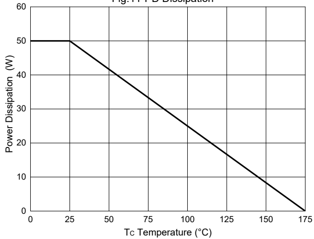
Fig.11-PD Dissipation
