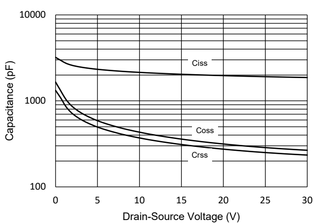
Fig.5-Capacitance Characteristics
