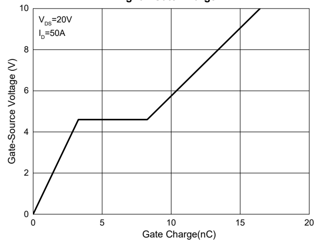
Fig. 6 - Gate Charge
