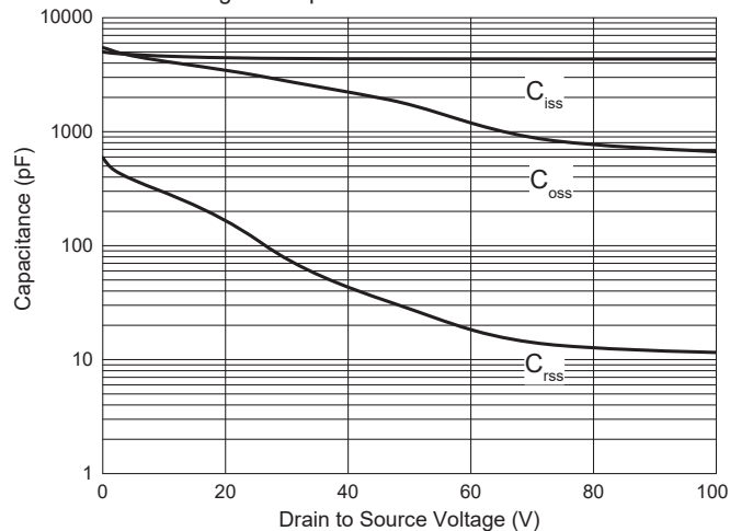
Fig. 5 - Capacitance Characteristics
