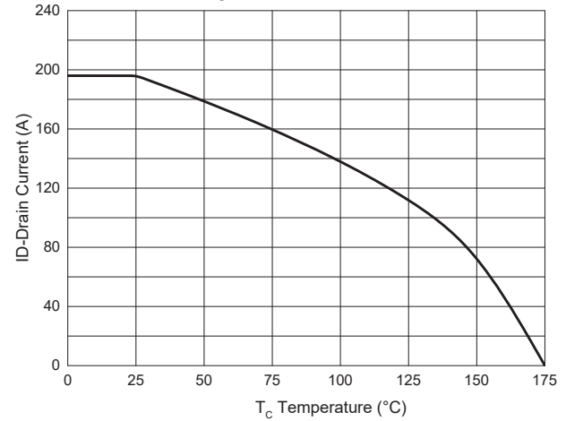
Fig. 10 - Drain Current
