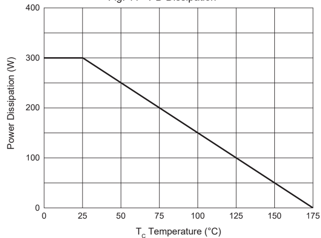
Fig. 11 - PD Dissipation
