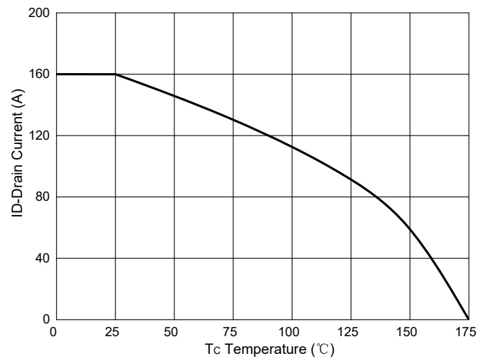
Fig. 10 - Drain Current
