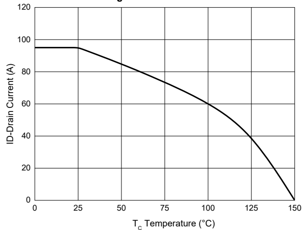
Fig. 10 - Drain Current
