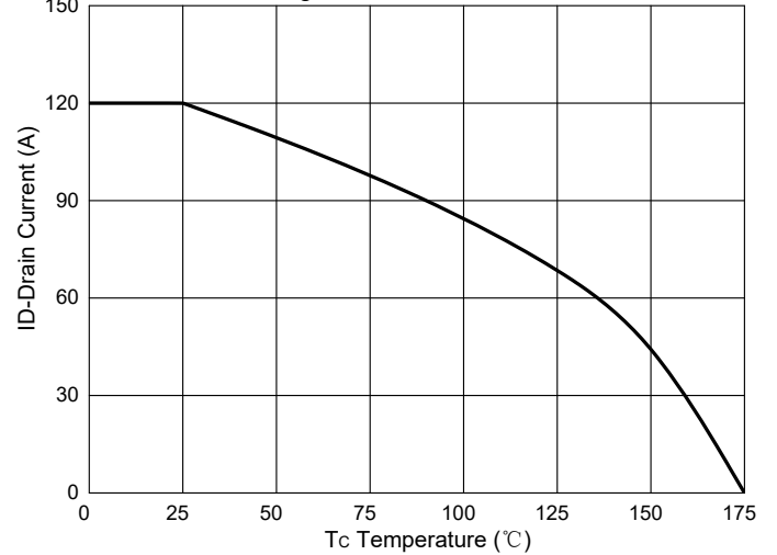
Fig. 10 - Drain Current
