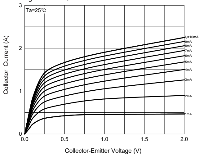
Fig. 1 - Static Characteristics
