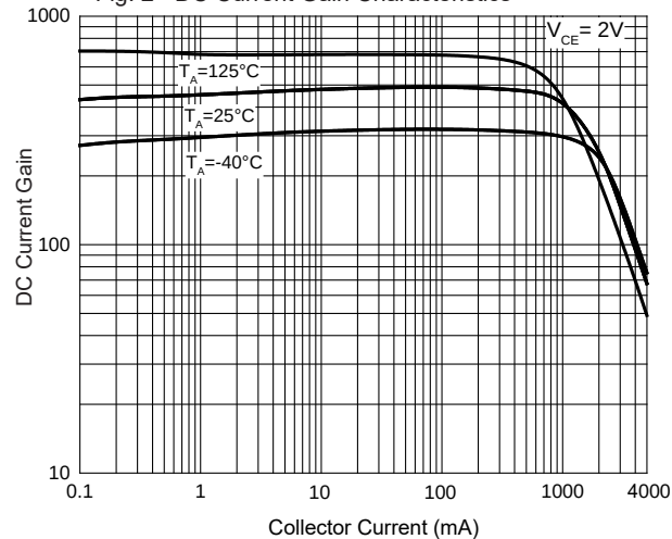
Fig. 2 - DC Current Gain Characteristics
