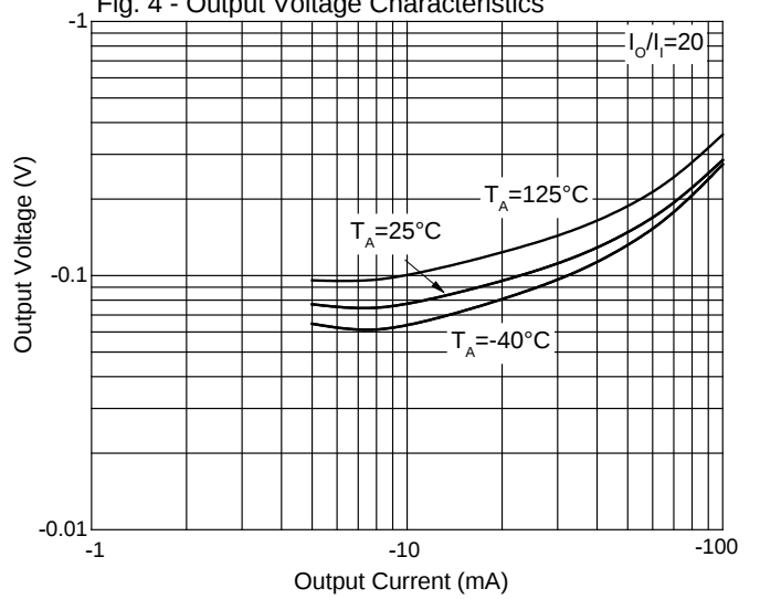
Fig. 4 - Output Voltage Characteristics
