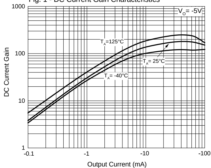
Fig. 1 - DC Current Gain Characteristics
