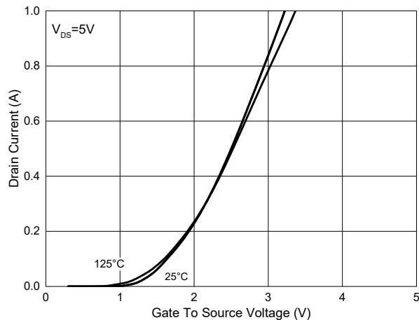
Fig.2 - Transfer Characteristic
