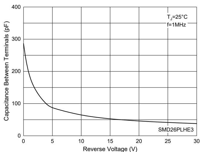
Fig. 10 - Capacitance Characteristics
