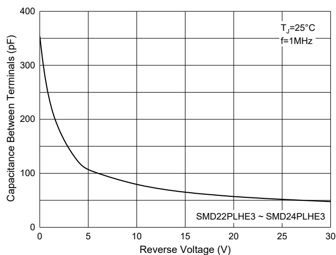
Fig. 9 - Capacitance Characteristics
