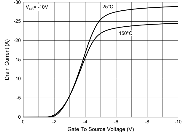
Fig. 2 - Transfer Characteristics
