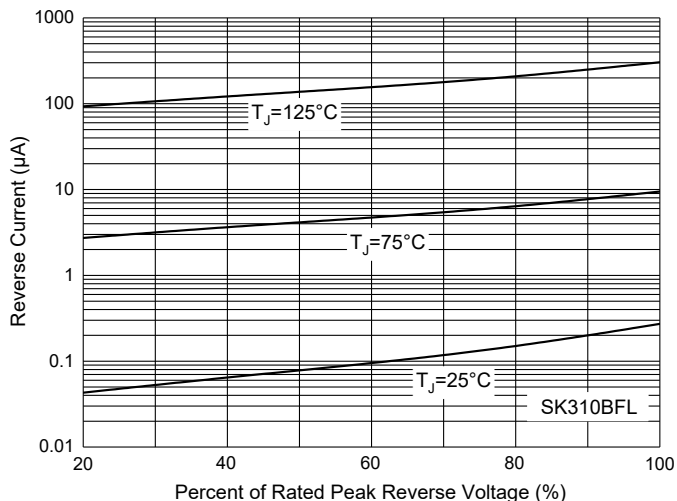
Fig. 9 - Typical Reverse Leakage Characteristics
