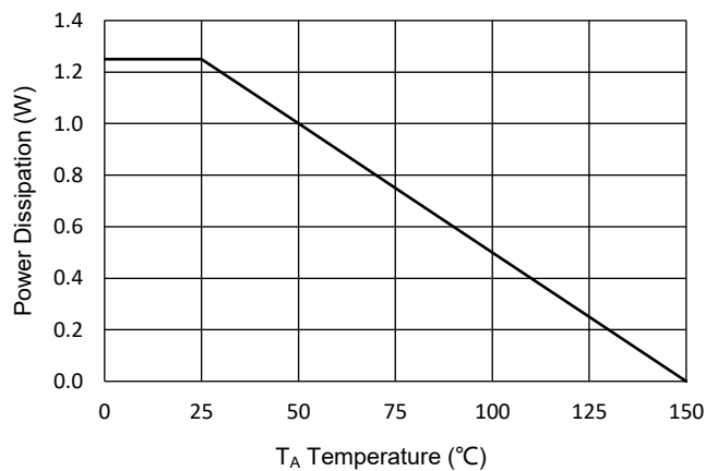
Fig.11 Power Dissipation
