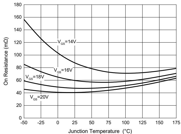
Fig. 5 On-Resistance vs Temperature
