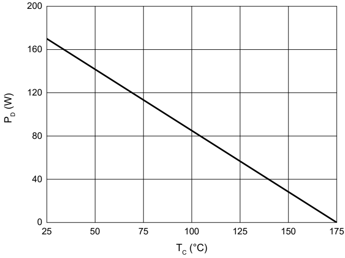
Fig. 7 - Power Derating
