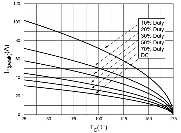
Fig. 4 - Current Derating
