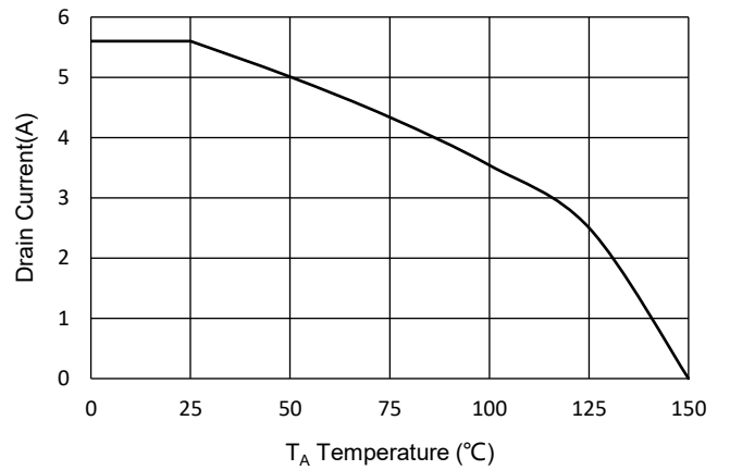
Fig.10 - Drain Current
