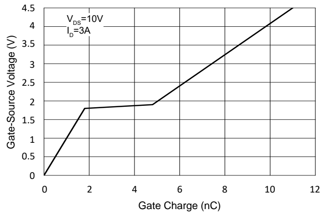
Fig.6 - Gate Charge
