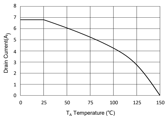
Fig.10 - Drain Current
