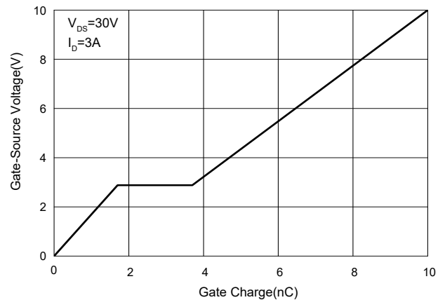
Fig. 6 - Gate Charge
