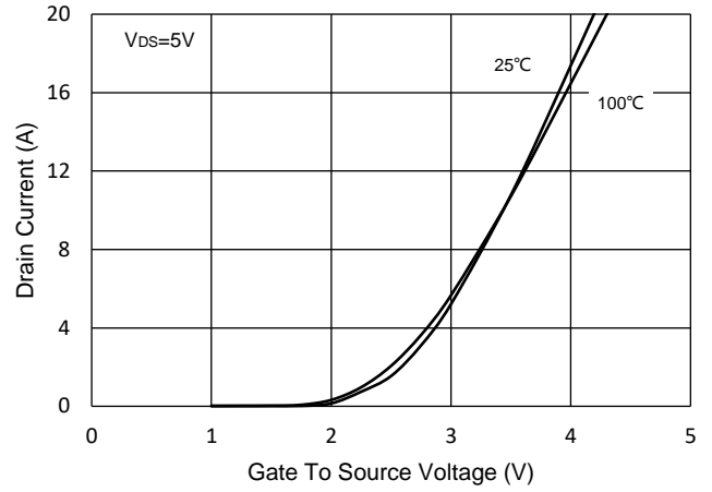
Fig.2 - Transfer Characteristic
