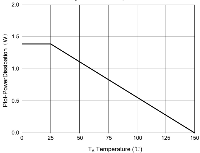
Fig.11-PowerDissipation
