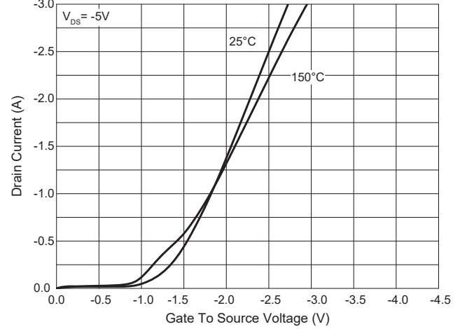
Fig. 2 - Transfer Characteristics
