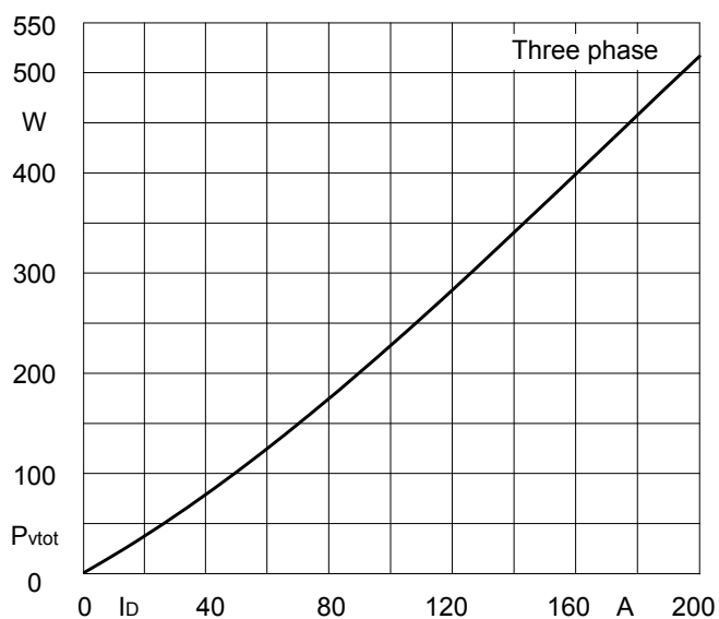
Fig1. Power dissipation
