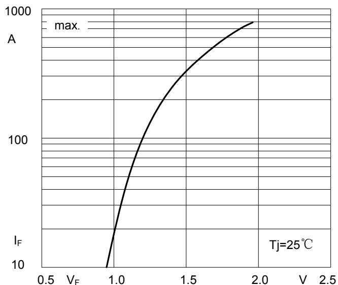
Fig5. Forward Characteristics
