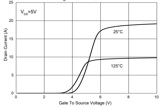
Fig. 2 - Transfer Characteristics
