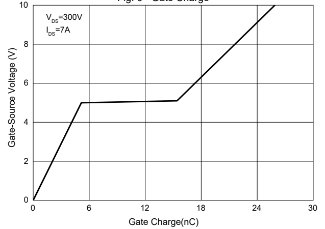
Fig. 6 - Gate Charge
