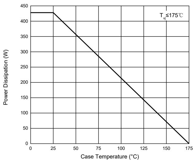
Fig. 18 - Power Derating
