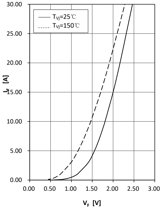
Fig13.Diode-brake-chopper Forward Characteristics
