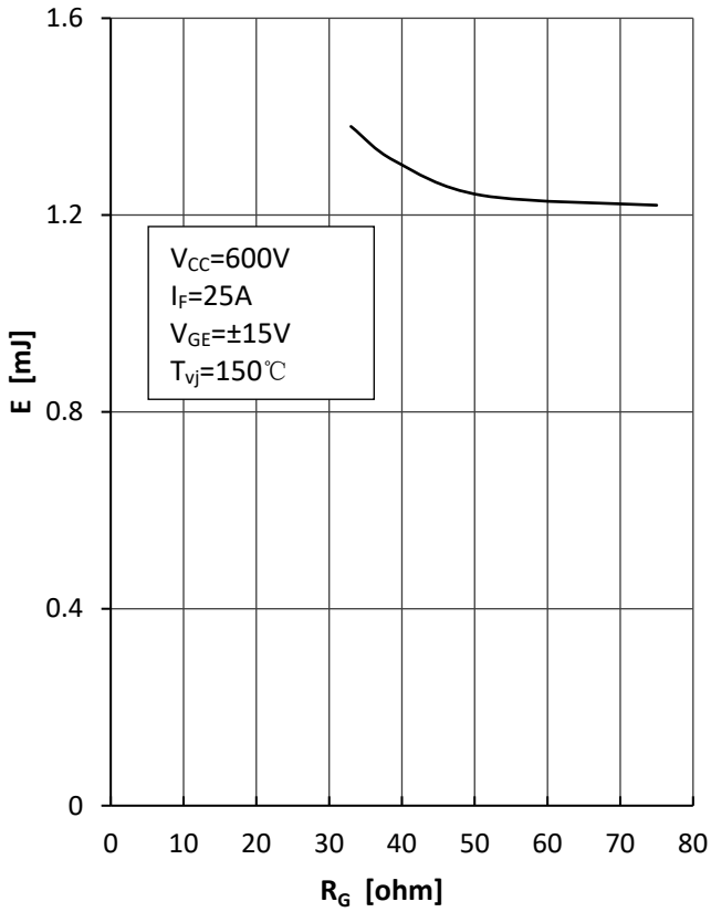
Fig9.Diode Switching Loss(Erec)vs.Rg
