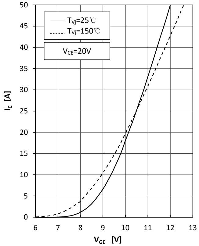
Fig2.IGBT Transfer Characteristics
