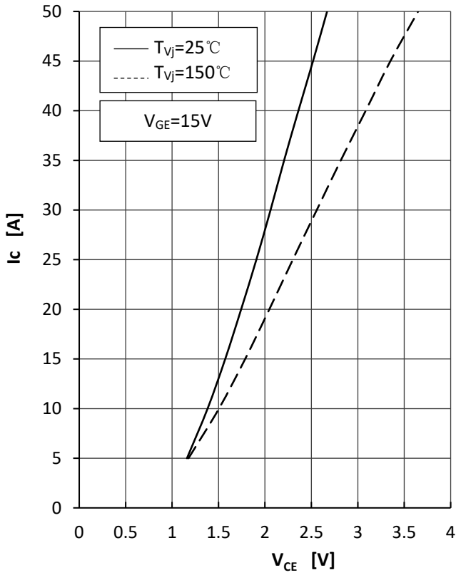
Fig1.IGBT Output Characteristics
